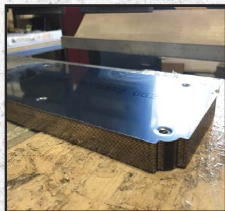
Blanks ready for bending machine
