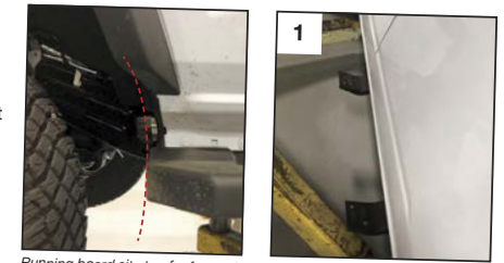
Running board sits too far forward into the wheel well
