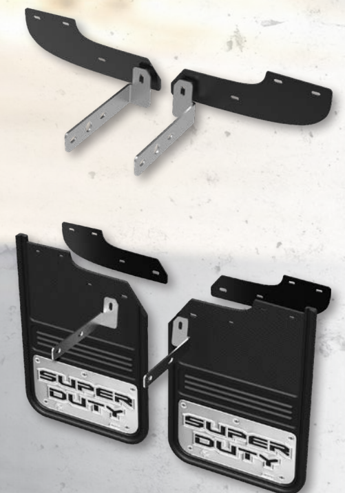
FRONT F450/550 MUDFLAP WITH BRACKET
