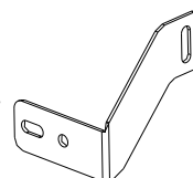
(1) Bracket Front, PS Part #769804
