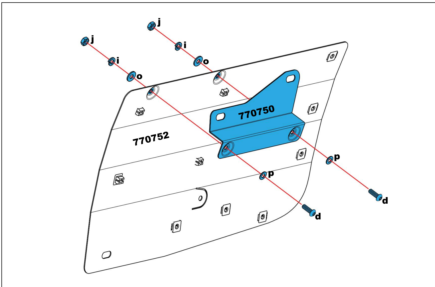
4-3 Install upper bracket to backing plate as shown
