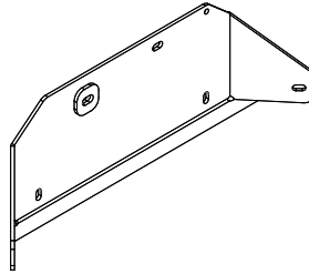
(1) Front Mount Part #702515
